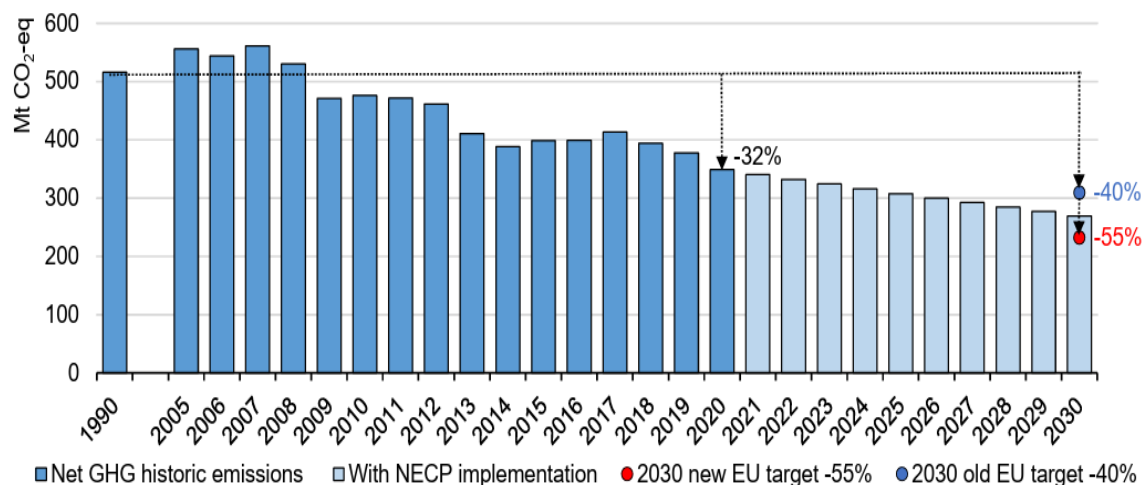
Figure 29: Italy's historic net greenhouse gas emissions, projections and 2030 targets [109]
